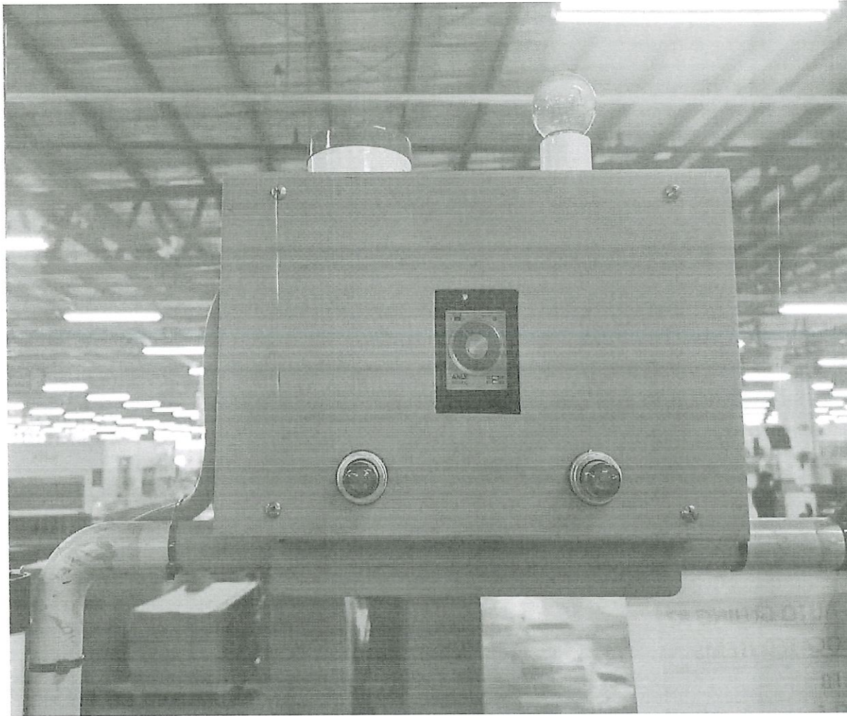
Alarm system installed for semi auto gluing machine
